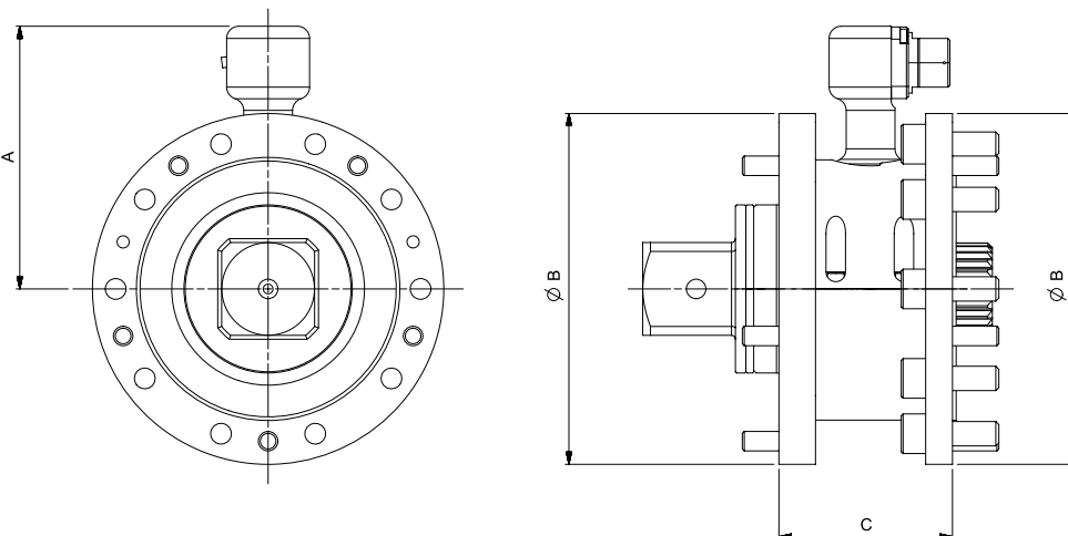
Fixed Connector
