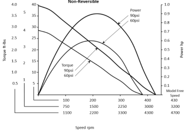
22M Speed Torque Data Non-Reversible
